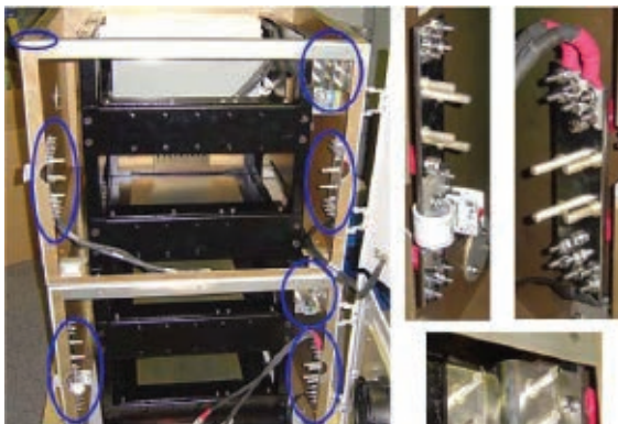
Chassis showing application of Plastic SurLok
